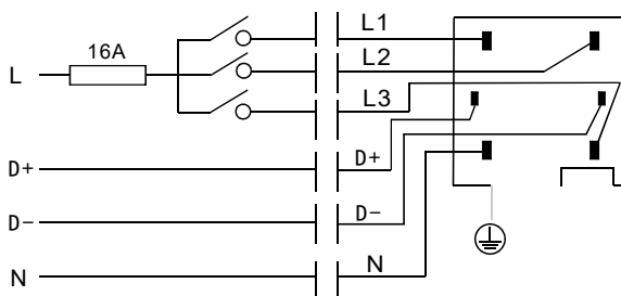
1 Phase 230VAC 16A Max + DALI
