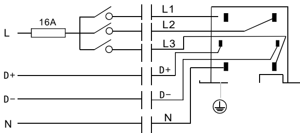
1 Phase 230VAC 16A Max + DALI
