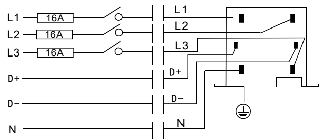
3 Phases 230VAC 3x16A Max + DALI
