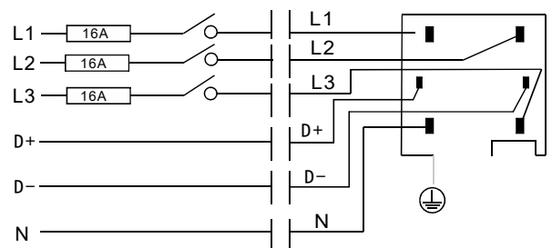
3 Phases 230VAC 3x16A Max + DALI
